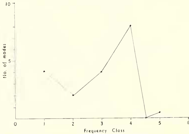
TEXT-FIG. 5. Plot of modal number of frequency class, of species in Newport and Gosford Bay assemblages. Explanation in text.
